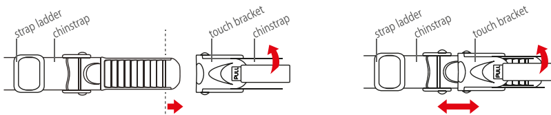
Quick-release retention system
